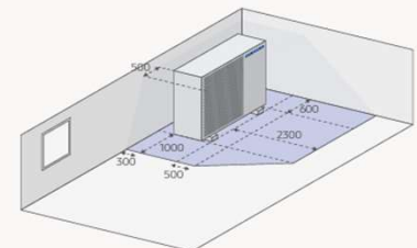
When installed at the right corner of a building
