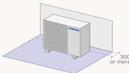
Wall on suction side
