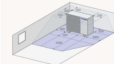
When installed at the left corner of a building
