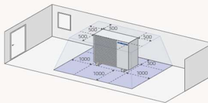
When installed on the ground on the front of the building wall
