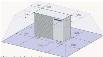
When installed on the ground when installed in a place with a flat roof
